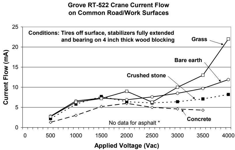
Figure 7 Current flow through the Grove RT-522 crane, tires off surface, on fully extended stabilisers bearing on 4 inch thick wood blocking, on four different surfaces. * Based on data for the RT-522 on tyres only, current flow through wood blocking support on asphalt would have been lower than that on all other surfaces.
