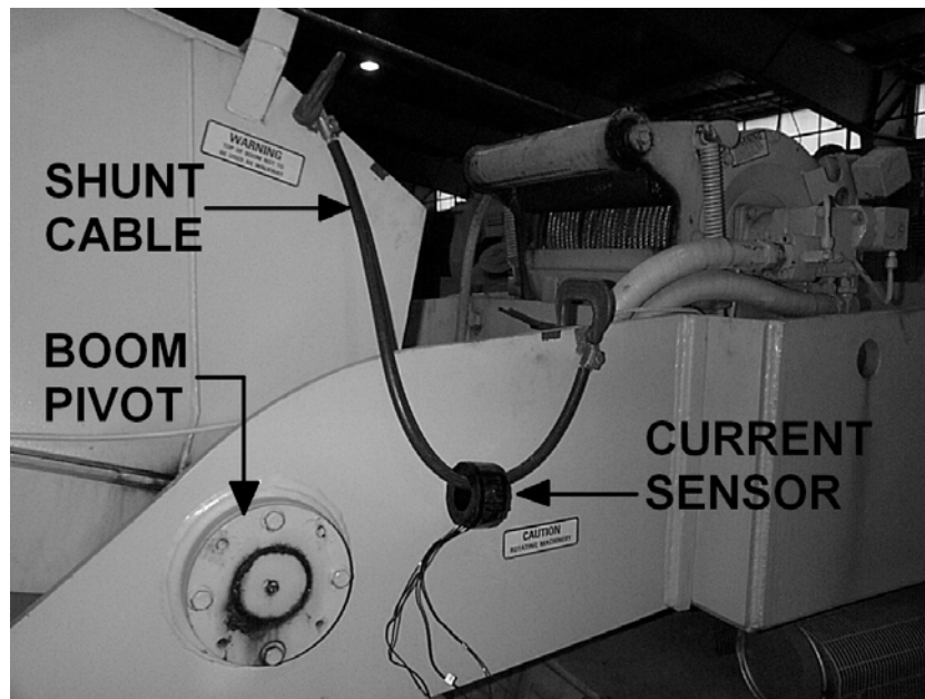
Figure 4 Shunt conductor with current transformer, bridging the main boom pivot on the Grove RT-522 crane.
