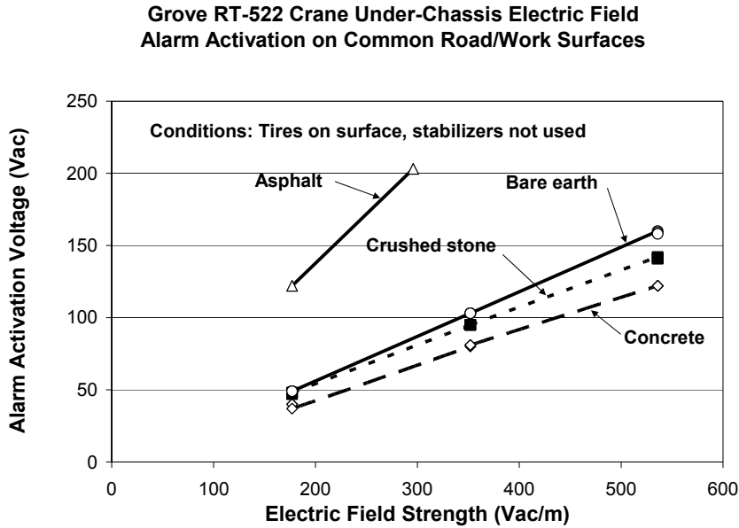
Figure 9 Alarm activation voltages (chassis voltages) for under-chassis electric field measurement, on the Grove RT-522 crane, on tires only, on four different surfaces. Multiple data points for each surface type represent different alarm circuitry sensitivity settings.
