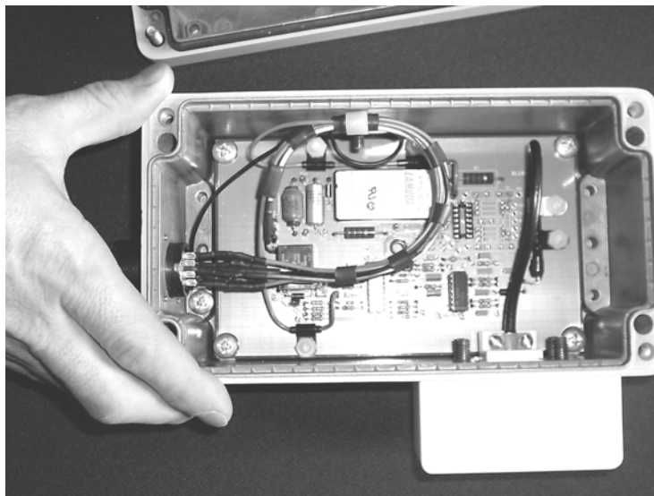
Figure 12 Electric field measurement sensor assembly for the prototype power line contact alarm system.
