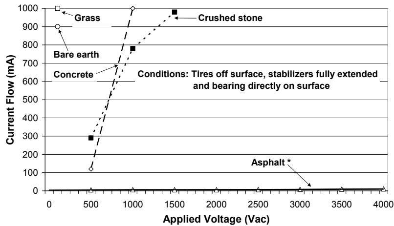
Figure 6 Current flow through the Grove RT-522 crane, tyres off surface, on fully extended stabilisers bearing directly on five different surfaces. * On asphalt, stabilisers were only in light contact.
