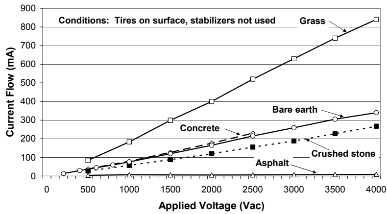
Figure 5 Current flow through the Grove RT-522 crane, on tyres only, on five different surfaces.
