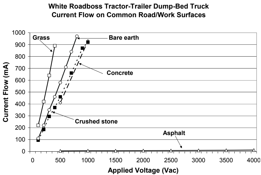
Figure 8 Current flow through the White Roadboss tractor-trailer dump-bed truck, on five different surfaces.
